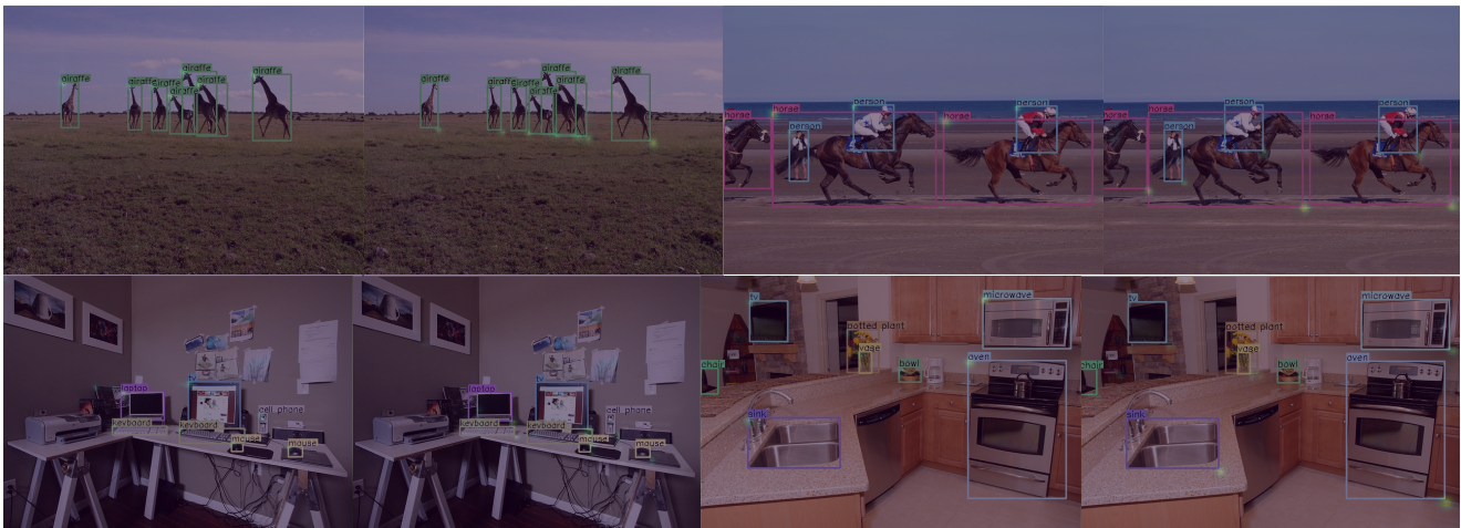
Fig. 10 Example bounding box predictions overlaid on predicted heatmaps of corners.
