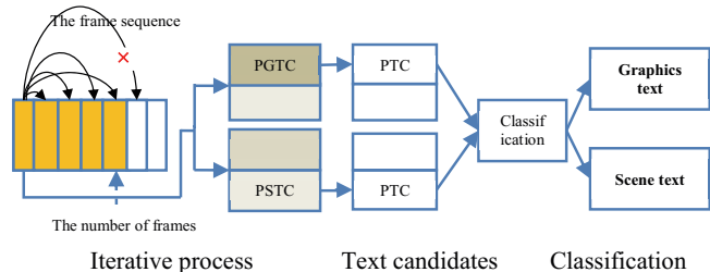
Fig. 1. Block diagram of the proposed classification method
