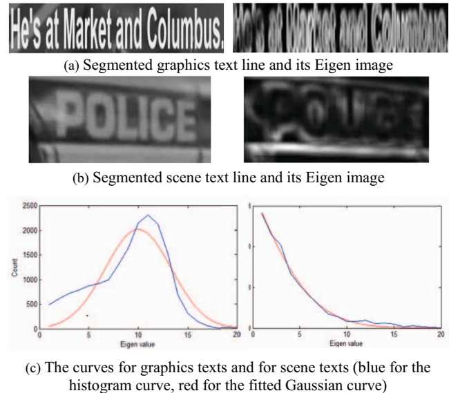
Fig. 5. Eigen value analysis for studying distribution of text pixels of both graphics and scene text
