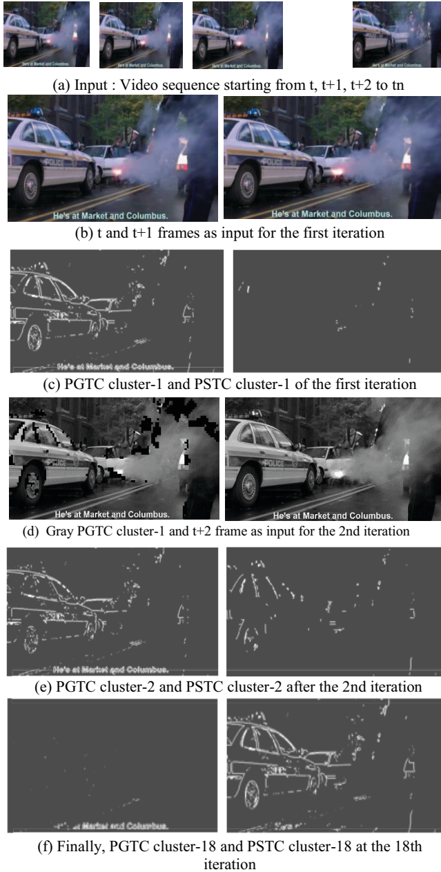
Fig. 2. Probable candidates of graphics and scene texts. Note that we shade the background of the cluster results to make visible
