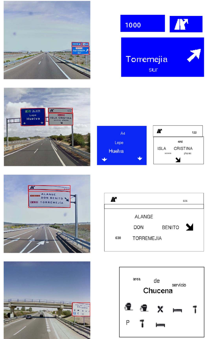
Fig. 11. Image results. Panel detections are on the left column and text recognition on the right column.
