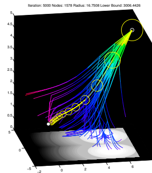
Fig. 8. The search tree for Light-Dark after 5000 iterations of planning. The belief space is represented in 3-dimensions, where the mean of the agent’s location estimate is the “floor”, and the vertical axis represents the variance of the agent’s belief distribution; lower points represent less location uncertainty. The algorithm builds a search tree to find a trajectory through belief-space. The optimized solution is shown as a thick yellow line, where the agent moves towards the goal while lowering the variance of its location distribution (descending the vertical axis). Policies in the tree are false-colored (green through magenta) as cost increases.
