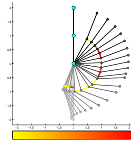
Fig. 4. A solution found after 5000 iterations of LQR-RRT* on the acrobot. Earlier state configurations are shown in lighter gray. Torque is presented as a false-colored arc where red represents higher values.
